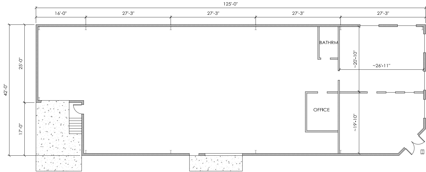
SCALE: 1/16" = 1'-0" (printed on 8.5"x11")
